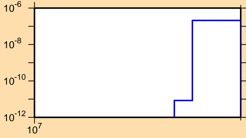
\sigma vs. E for ^{123}\text{Sb}(n,2np)
