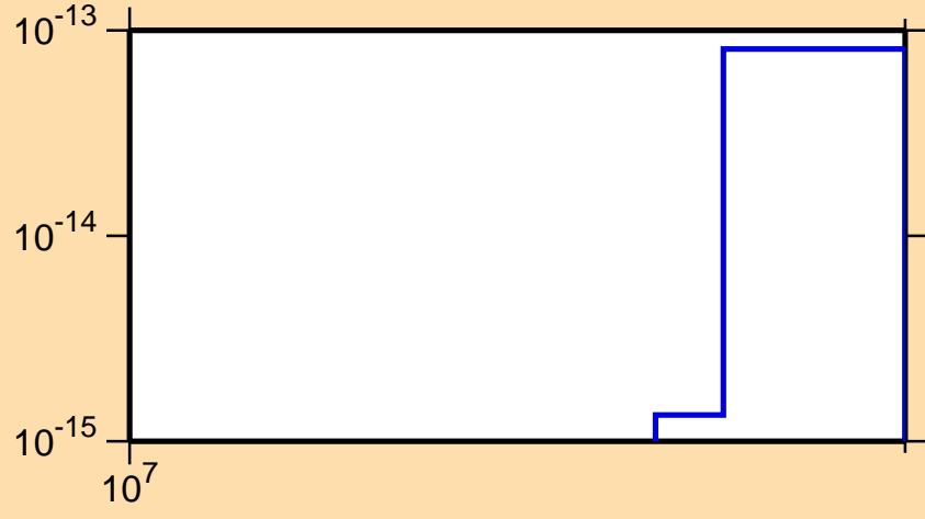
\sigma vs. E for ^{123}\text{Sb}(n,p\alpha)
