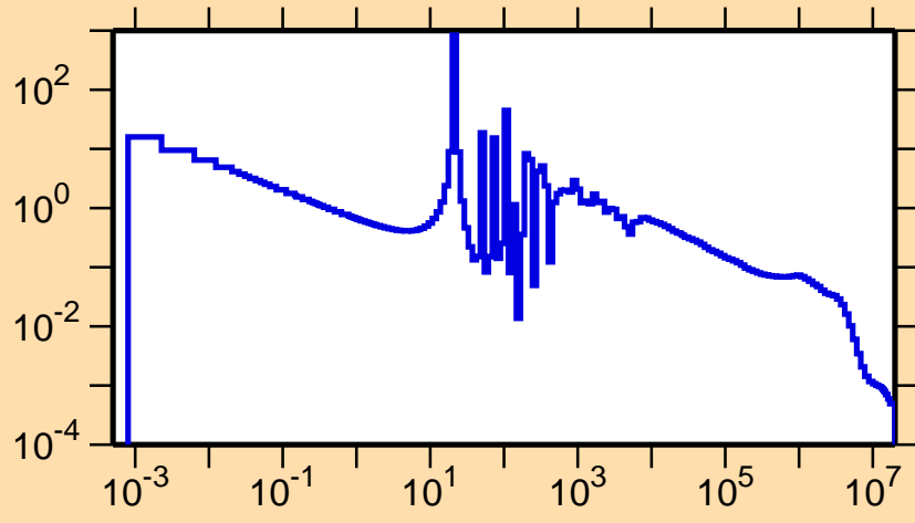
\sigma vs. E for ^{123}\text{Sb}(n,\gamma)
