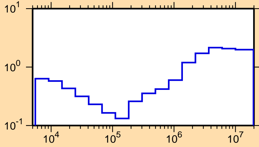
\sigma vs. E for ^{123}\text{Sb}(n,\text{nonel.})
