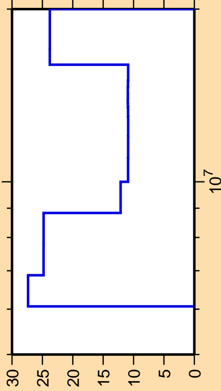
\Delta\sigma/\sigma vs. E for ^{124}\text{Sb}(n,2n)
