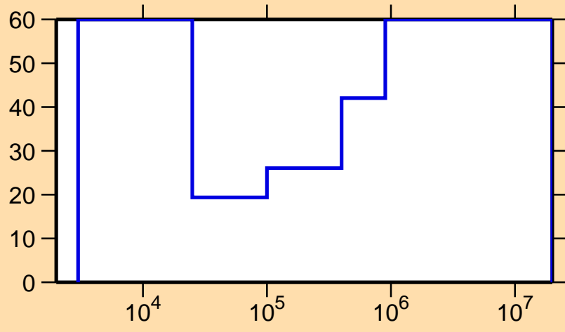
\Delta\sigma/\sigma vs. E for ^{124}\text{Sb}(n,n_1)
