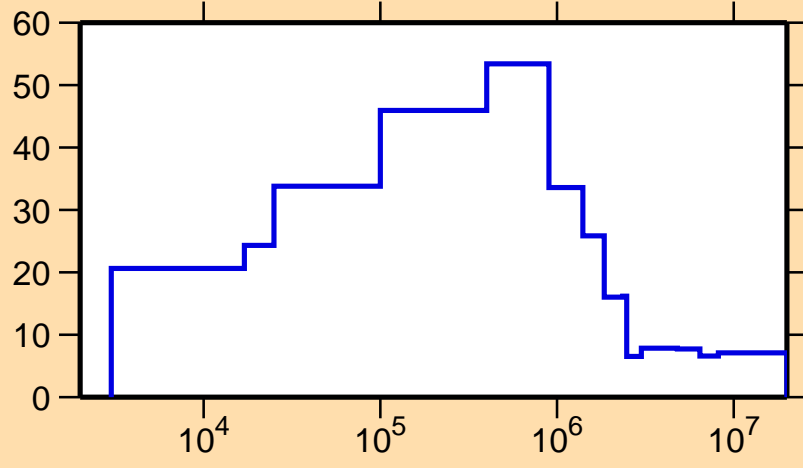
\Delta\sigma/\sigma vs. E for ^{124}\text{Sb}(n,\text{nonel.})
