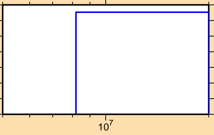
\sigma vs. E for ^{124}\text{Sb}(n,nt)
