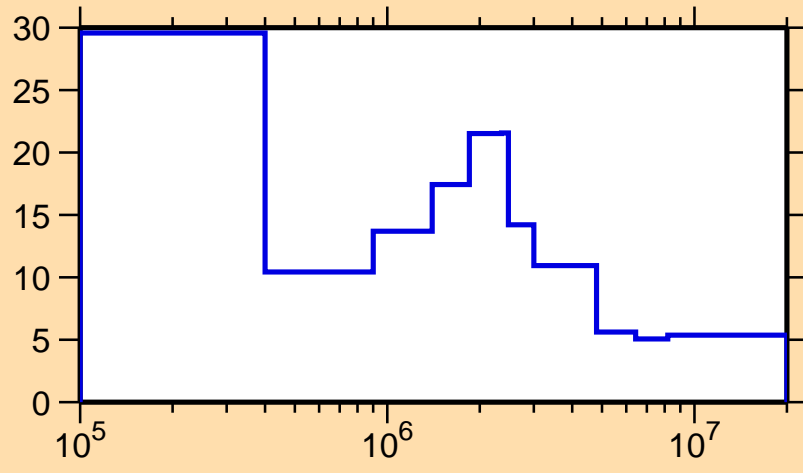
\Delta\sigma/\sigma vs. E for ^{124}\text{Sb}(n,\text{tot.})
