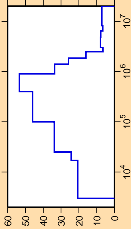
\Delta\sigma/\sigma vs. E for ^{124}\text{Sb}(n,\text{nonel.})
