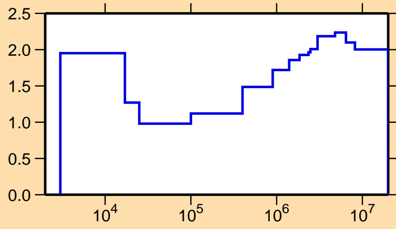
\sigma vs. E for ^{124}\text{Sb}(n,\text{nonel.})
