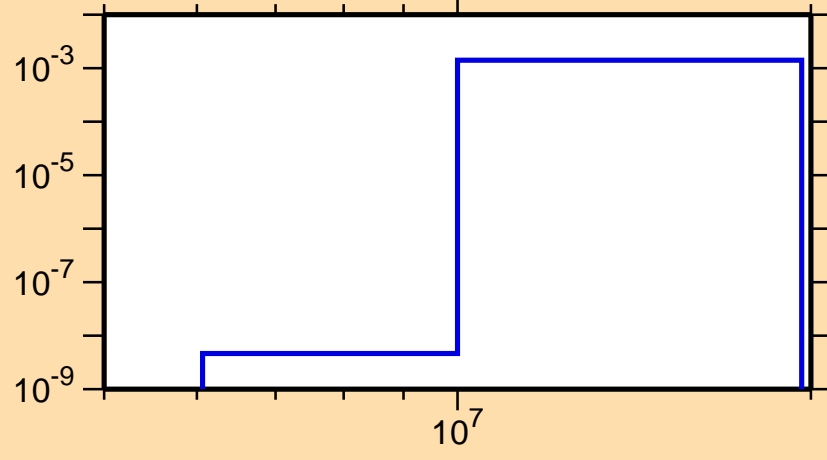
\sigma vs. E for ^{124}\text{Sb}(n,np)
