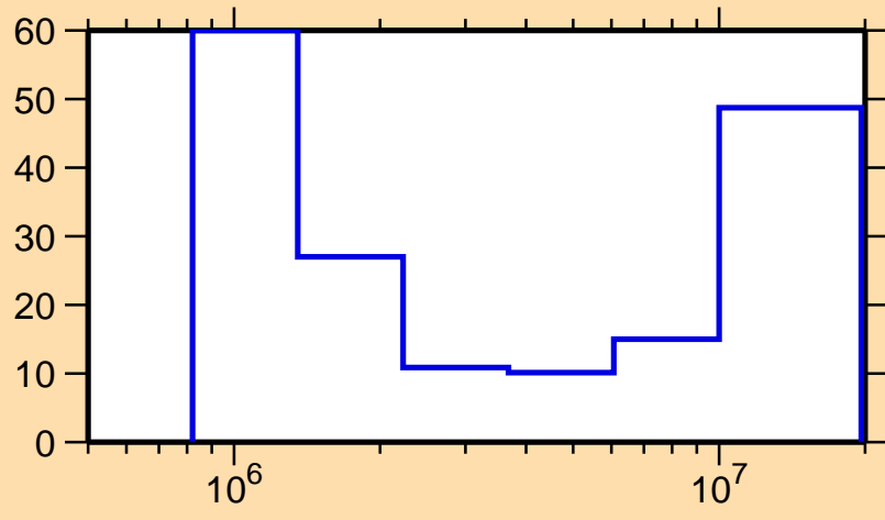
\Delta\sigma/\sigma vs. E for ^{124}\text{Sb}(n,n\text{cont.})
