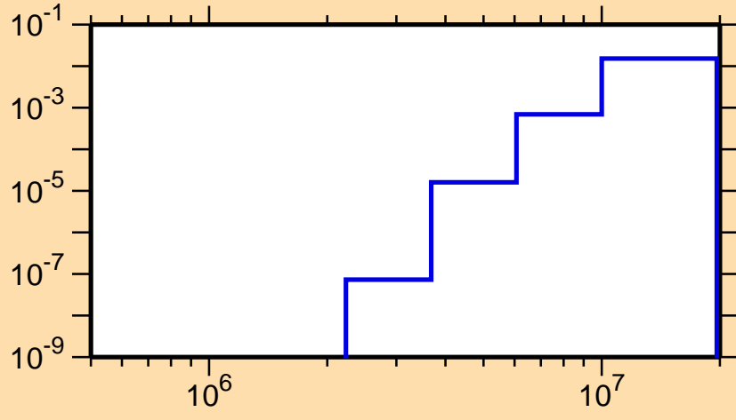
\sigma vs. E for ^{124}\text{Sb}(n,p)
