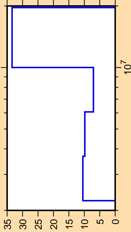
\Delta\sigma/\sigma vs. E for ^{125}\text{Sb}(n,n\text{cont.})
