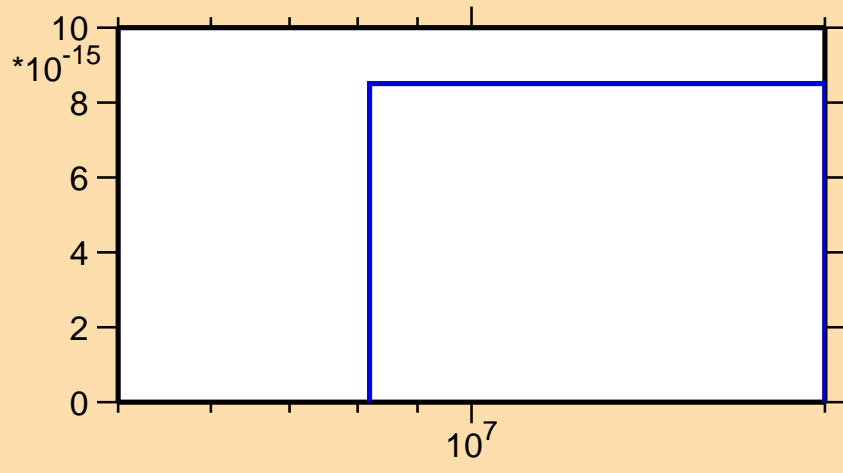
\sigma vs. E for ^{125}\text{Sb}(n,\text{He}3)
