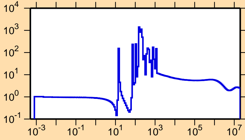
\sigma vs. E for ^{126}\text{Sb}(n,\text{el.})
