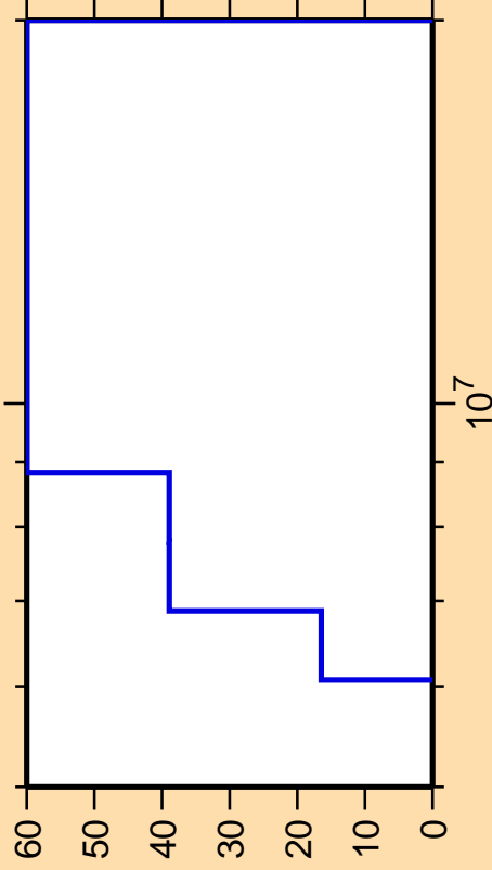
\Delta\sigma/\sigma vs. E for ^{126}\text{Sb}(n,n\text{cont.})
