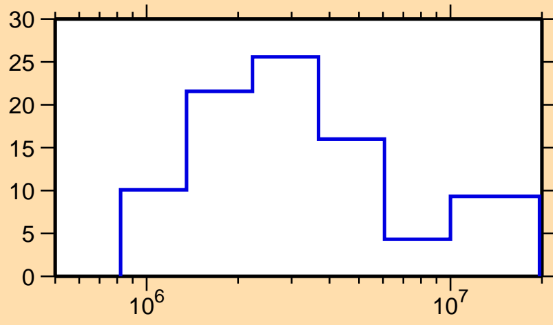
\Delta\sigma/\sigma vs. E for ^{126}\text{Sb}(n,el.)
