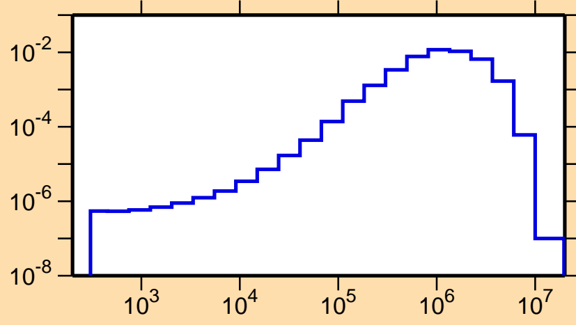
\sigma vs. E for ^{126}\text{Sb}(n,n_1)
