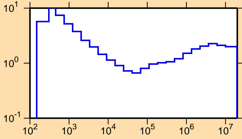
\sigma vs. E for ^{126}\text{Sb}(n,\text{nonel.})
