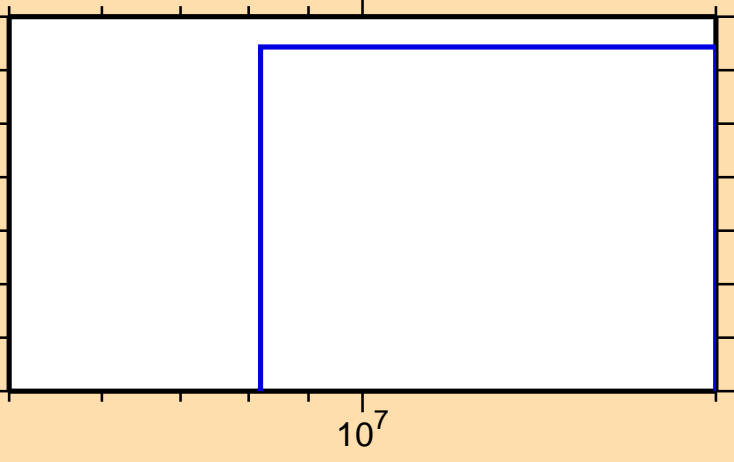
\sigma vs. E for ^{126}\text{Sb}(n,3n)
