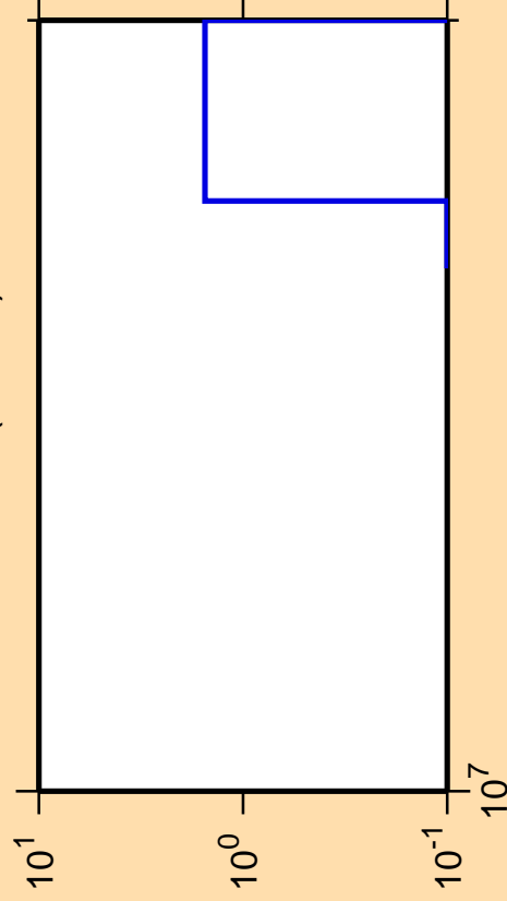
\Delta\sigma/\sigma vs. E for ^{127}\text{Sb}(n,2n\alpha)
