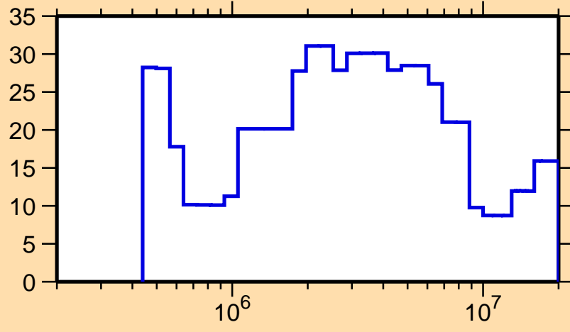
\Delta\sigma/\sigma vs. E for ^{127}\text{Sb}(n,\text{el.})
