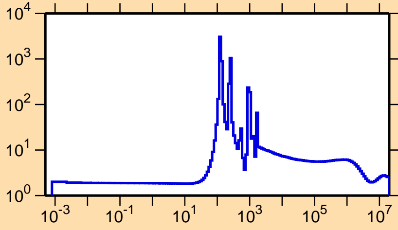
\sigma vs. E for ^{127}\text{Sb}(n,\text{el.})
