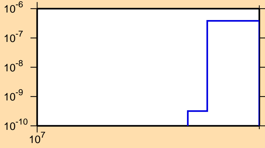
\sigma vs. E for ^{127}\text{Sb}(n,\text{nd})
