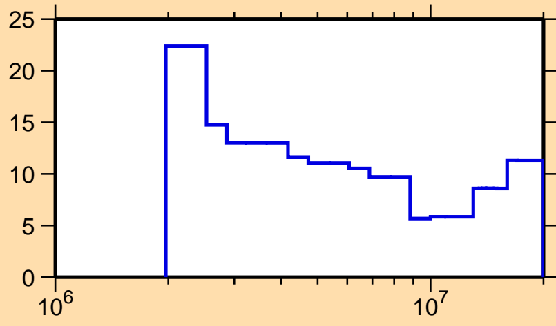
\Delta\sigma/\sigma vs. E for ^{127}\text{Sb}(n,\text{tot.})
