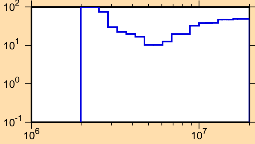
\Delta\sigma/\sigma vs. E for ^{127}\text{Sb}(n,n\text{cont.})
