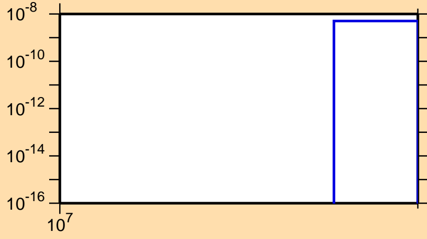
\sigma vs. E for ^{127}\text{Sb}(n,2np)
