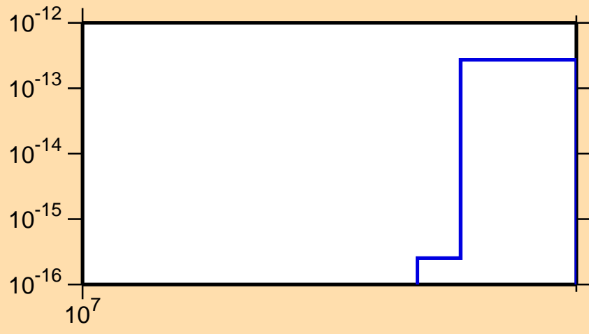
\sigma vs. E for ^{127}\text{Sb}(n,2n\alpha)
