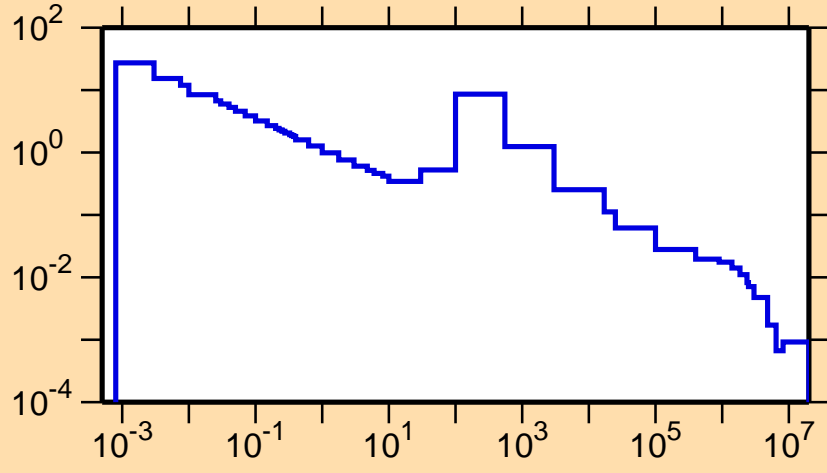
\sigma vs. E for ^{127}\text{Sb}(n,\gamma)
