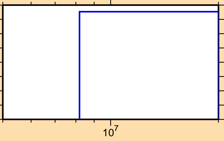
\sigma vs. E for ^{127}\text{Sb}(n,t)
