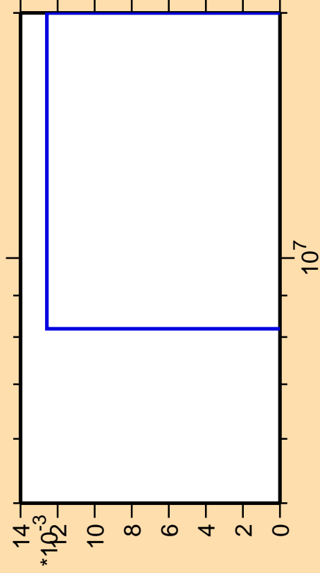
\Delta\sigma/\sigma vs. E for ^{127}\text{Sb}(n,2n\alpha)
