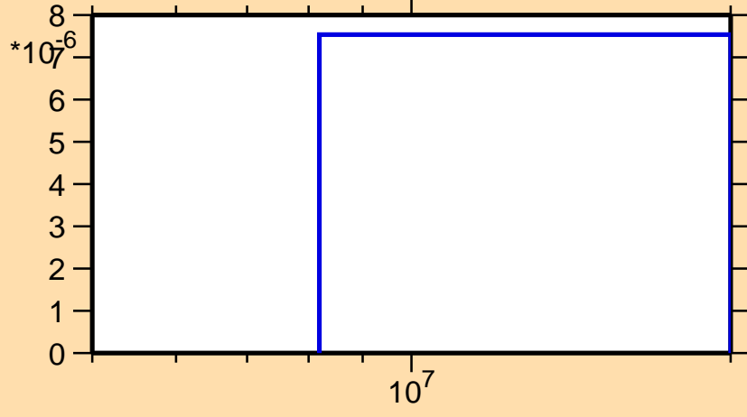
\sigma vs. E for ^{127}\text{Sb}(n,t)
