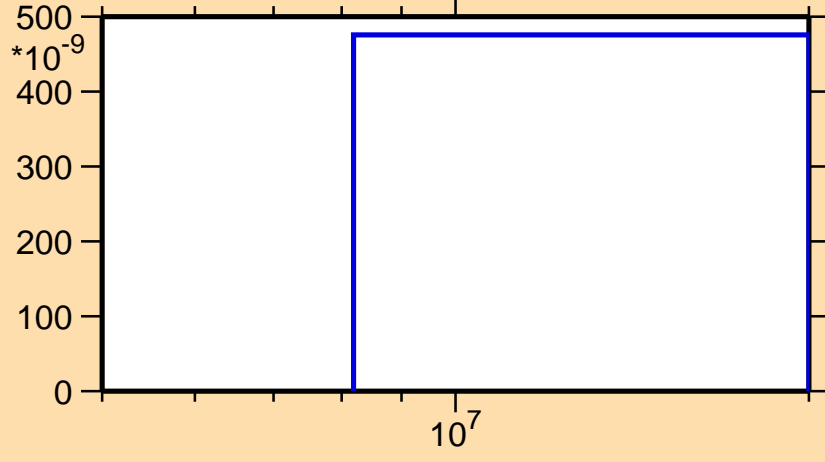
\sigma vs. E for ^{127}\text{Sb}(n,n\alpha)
