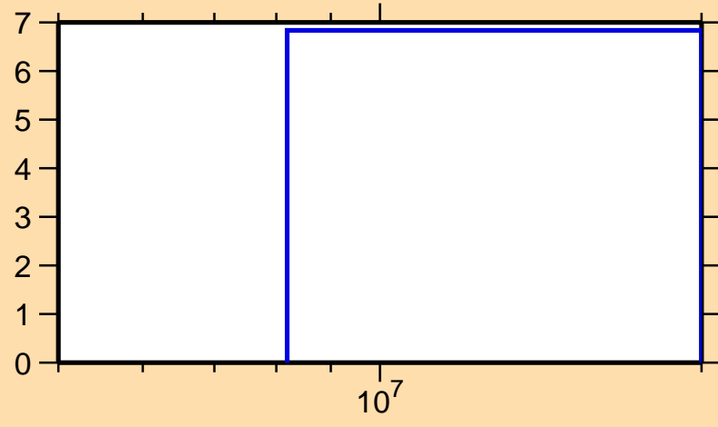
\Delta\sigma/\sigma vs. E for ^{127}\text{Sb}(n,\text{tot.})
