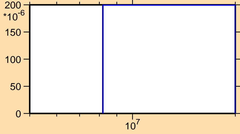
\sigma vs. E for ^{127}\text{Sb}(n,np)
