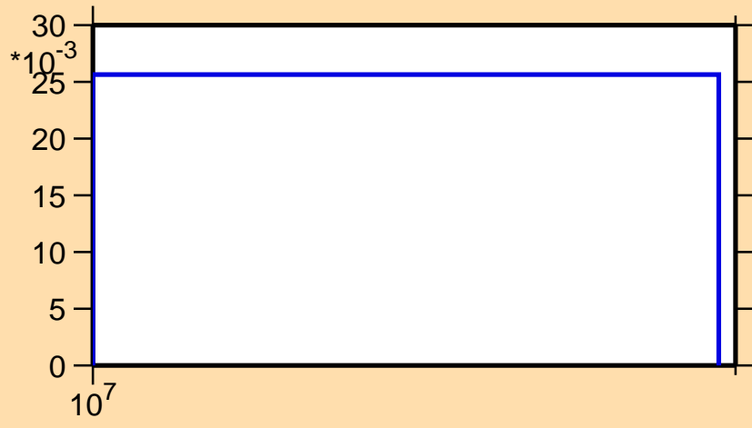
\sigma vs. E for ^{128}\text{Sb}(n,3n)
