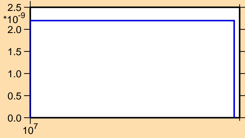
\sigma vs. E for ^{128}\text{Sb}(n,nt)
