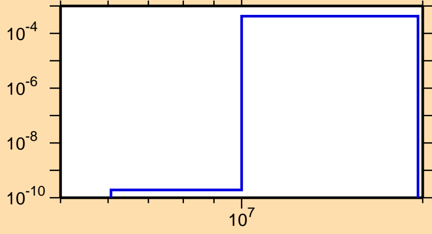
\sigma vs. E for ^{128}\text{Sb}(n,d)
