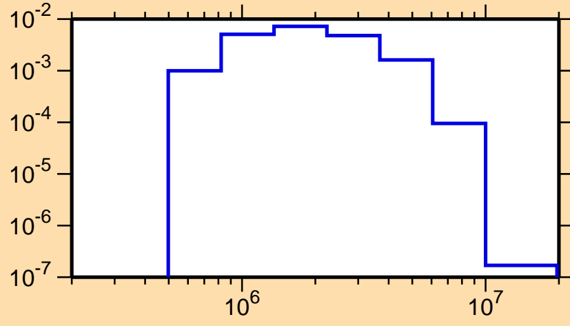
\sigma vs. E for ^{128}\text{Sb}(n,n_2)
