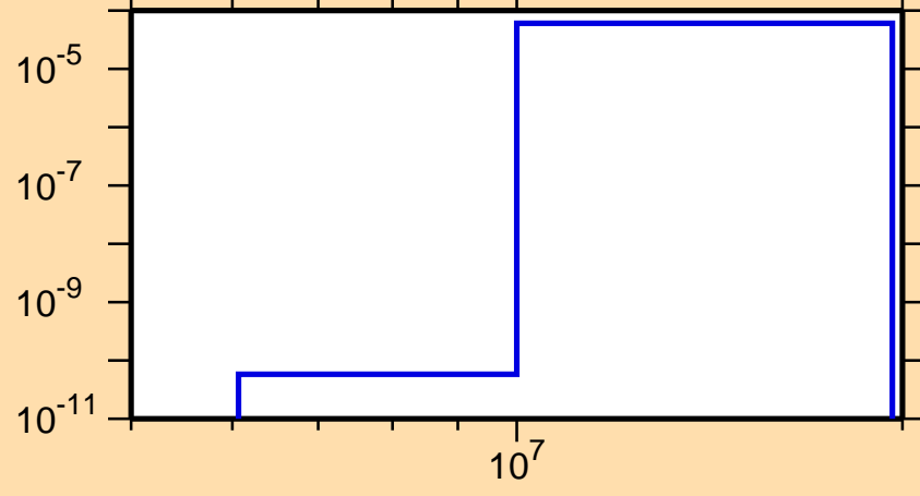
\sigma vs. E for ^{128}\text{Sb}(n,t)
