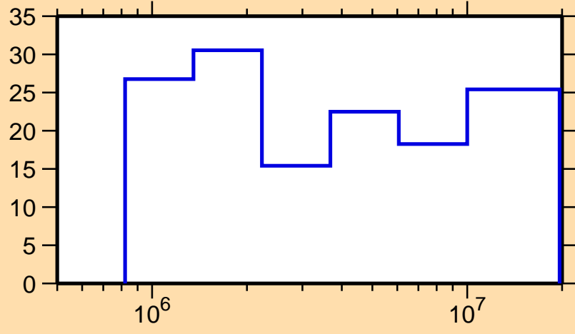
\Delta\sigma/\sigma vs. E for ^{128}\text{Sb}(n,el.)
