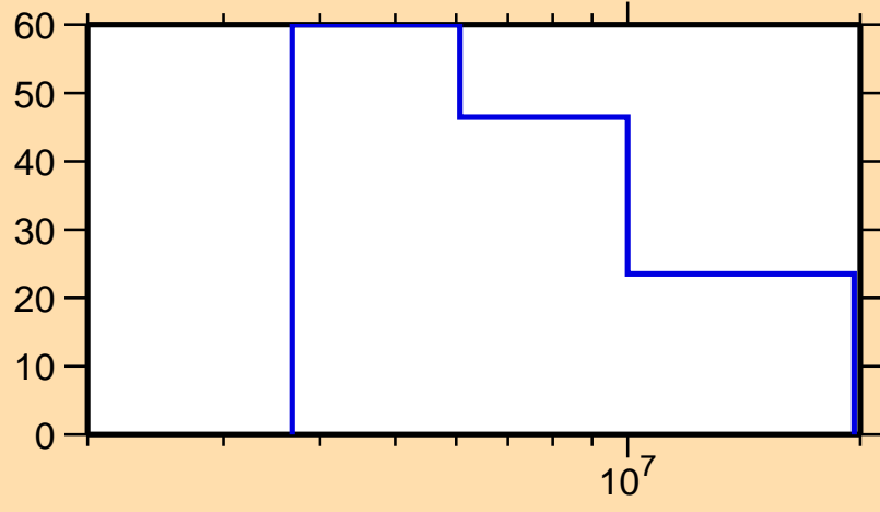
\Delta\sigma/\sigma vs. E for ^{128}\text{Sb}(n,2n)
