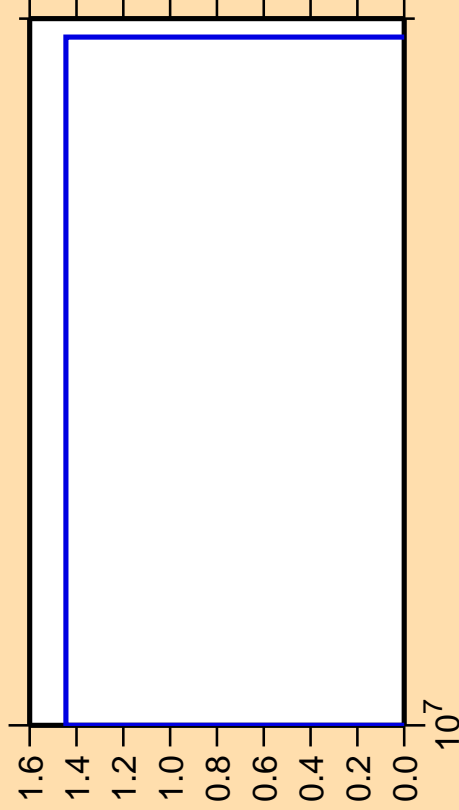
\Delta\sigma/\sigma vs. E for ^{128}\text{Sb}(n,2n\alpha)
