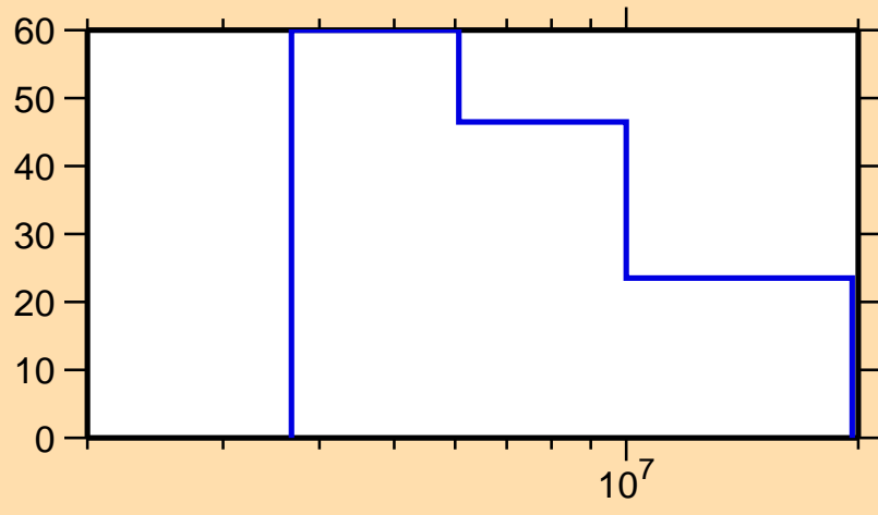
\Delta\sigma/\sigma vs. E for ^{128}\text{Sb}(n,2n)
