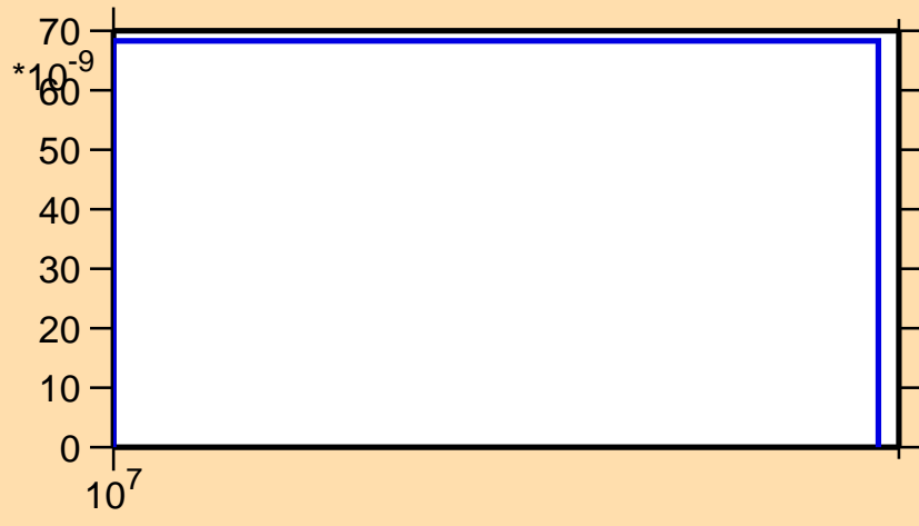
\sigma vs. E for ^{128}\text{Sb}(n,\text{nd})
