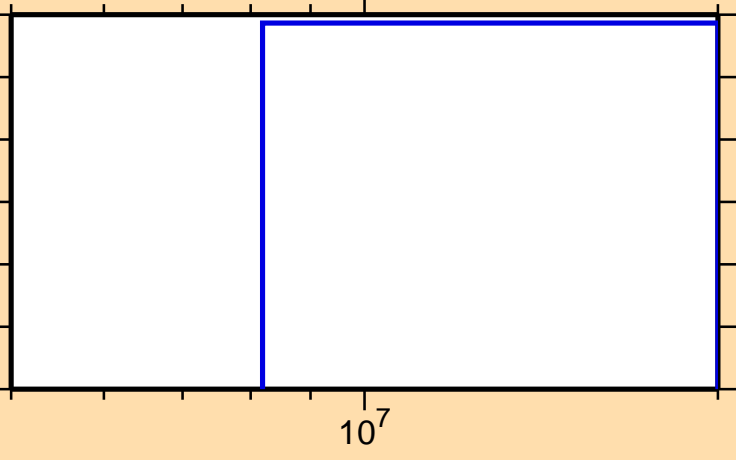
\sigma vs. E for ^{128}\text{Sb}(n,nd)
