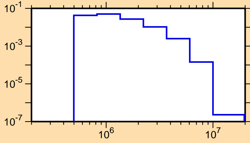
\sigma vs. E for ^{128}\text{Sb}(n,n_4)
