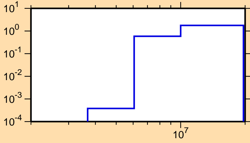
\sigma vs. E for ^{128}\text{Sb}(n,2n)
