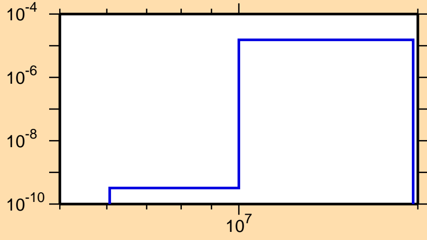
\sigma vs. E for ^{129}\text{Sb}(n,\alpha)
