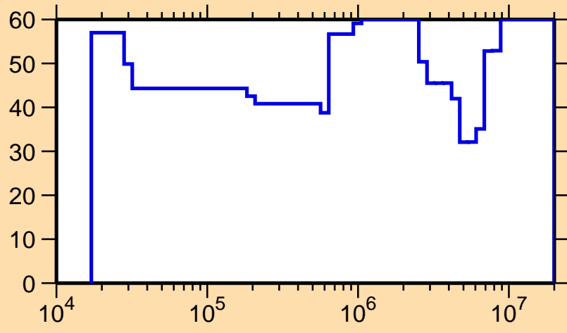
\Delta\sigma/\sigma vs. E for ^{129}\text{Sb}(n,n_1)
