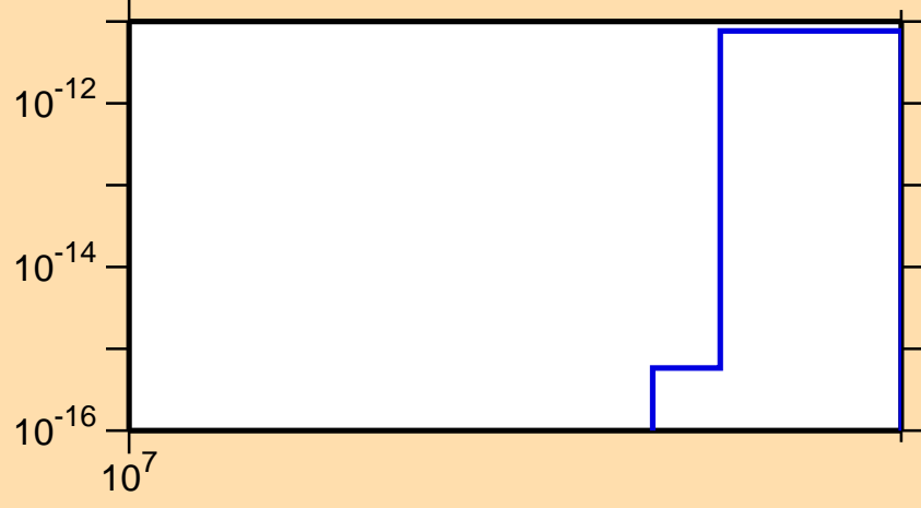
\sigma vs. E for ^{129}\text{Sb}(n,2n\alpha)
