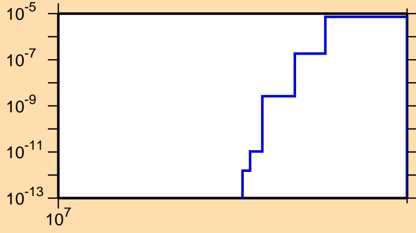
\sigma vs. E for ^{129}\text{Sb}(n,\text{nd})
