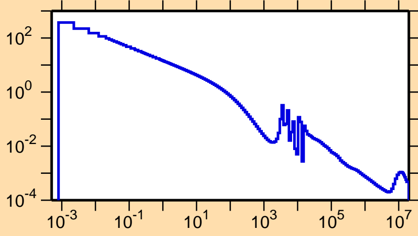
\sigma vs. E for ^{129}\text{Sb}(n,\gamma)
