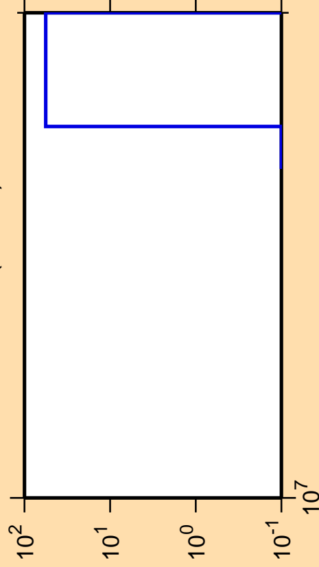
\Delta\sigma/\sigma vs. E for ^{129}\text{Sb}(n,2n\alpha)
