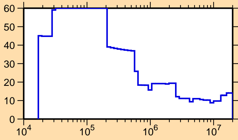
\Delta\sigma/\sigma vs. E for ^{129}\text{Sb}(n, \text{tot.})
