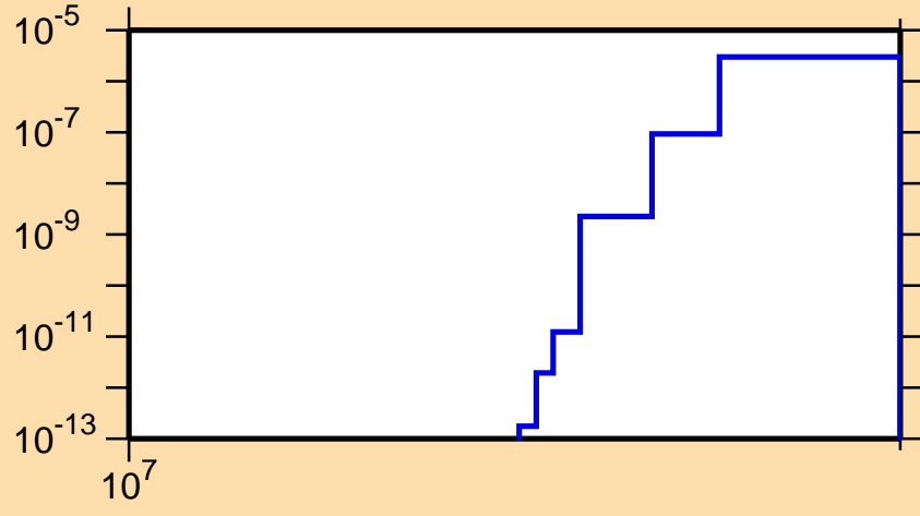
\sigma vs. E for ^{129}\text{Sb}(n,nt)
