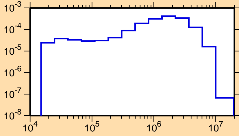
\sigma vs. E for ^{129}\text{Sb}(n,n_2)
