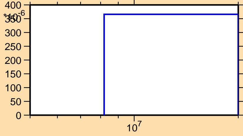
\sigma vs. E for ^{129}\text{Sb}(n,np)
