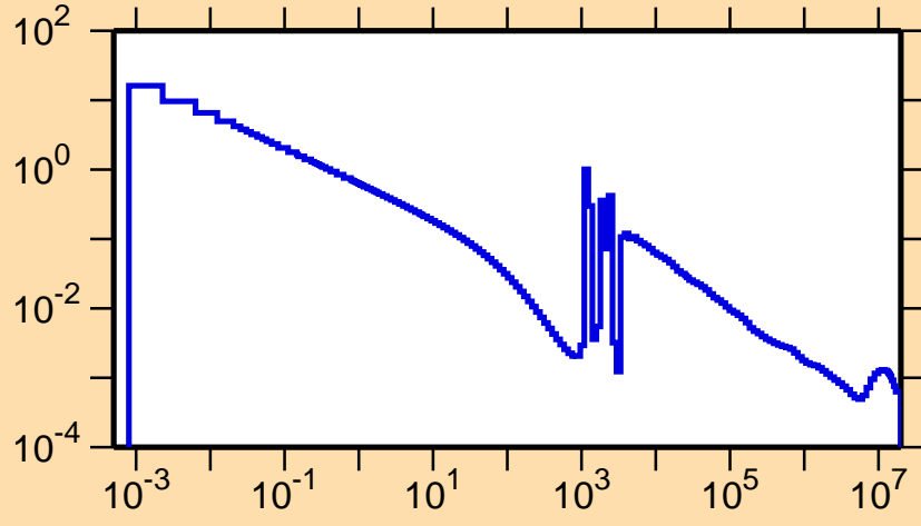
\sigma vs. E for ^{130}\text{Sb}(n,\gamma)
