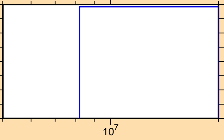
\sigma vs. E for ^{130}\text{Sb}(n,3n)
