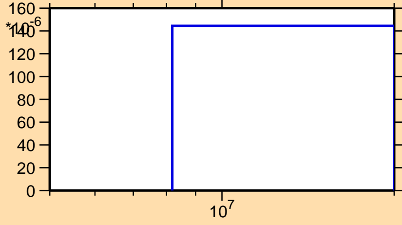
\sigma vs. E for ^{130}\text{Sb}(n,np)
