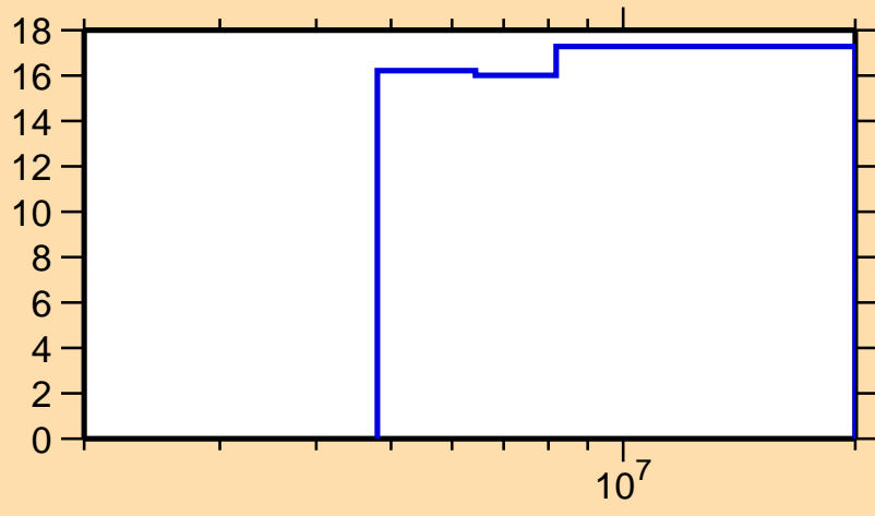
\Delta\sigma/\sigma vs. E for ^{130}\text{Sb}(n,\text{nonel.})
