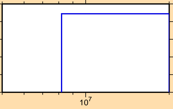
\sigma vs. E for ^{130}\text{Sb}(n,n\alpha)
