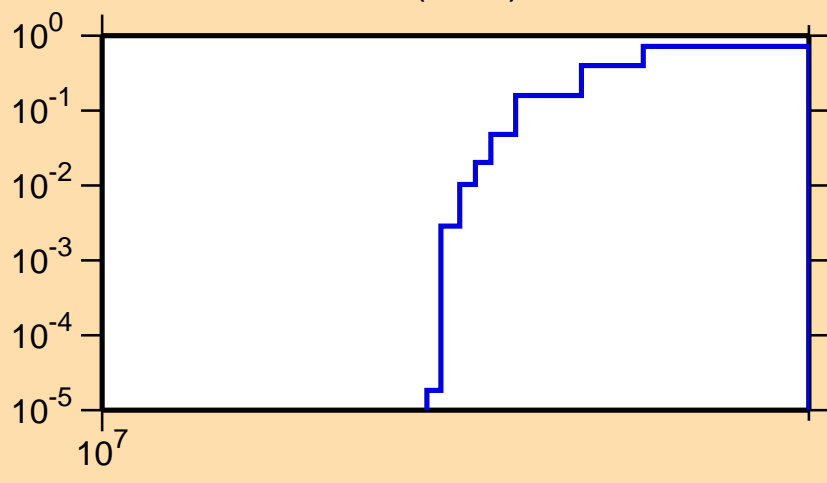
\sigma vs. E for ^{130}\text{Sb}(n,3n)
