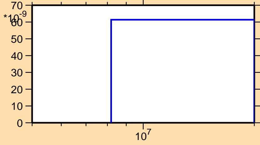
\sigma vs. E for ^{130}\text{Sb}(n,nd)
