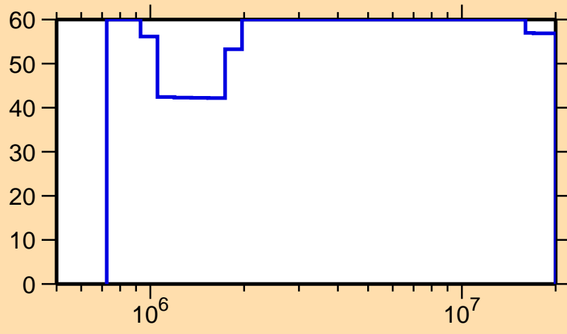
\Delta\sigma/\sigma vs. E for ^{131}\text{Sb}(n,n_1)
