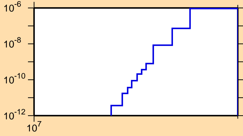
\sigma vs. E for ^{131}\text{Sb}(n,n\alpha)
