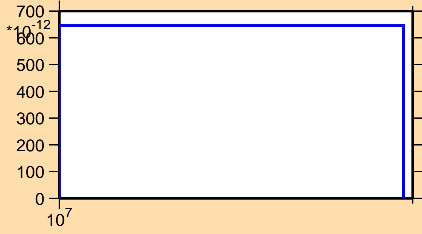
\sigma vs. E for ^{131}\text{Sb}(n,\text{nd})
