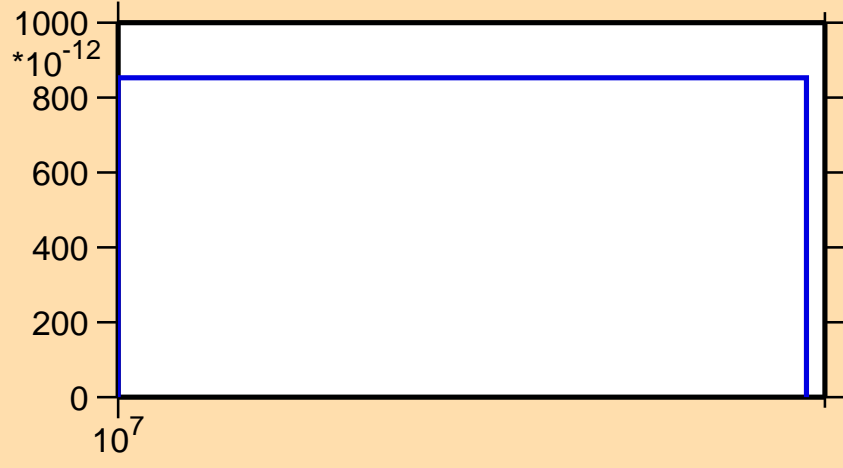
\sigma vs. E for ^{131}\text{Sb}(n,nt)
