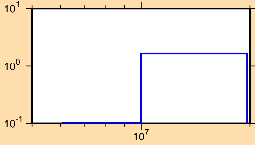
\sigma vs. E for ^{131}\text{Sb}(n,2n)
