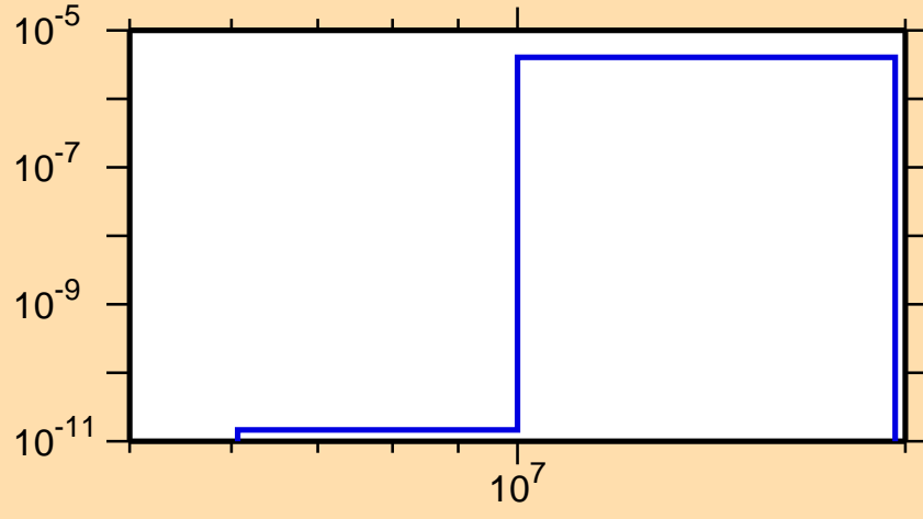
\sigma vs. E for ^{131}\text{Sb}(n,\alpha)
