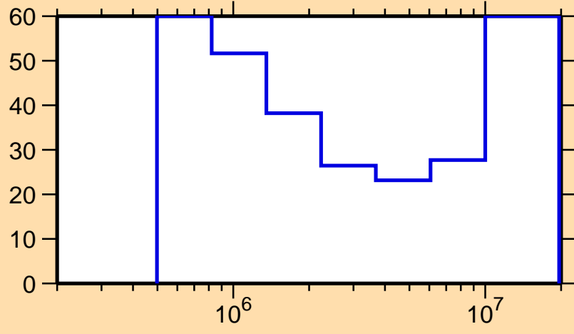
\Delta\sigma/\sigma vs. E for ^{131}\text{Sb}(n,\text{inel.})
