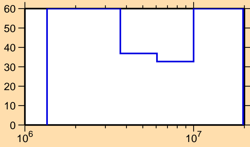
\Delta\sigma/\sigma vs. E for ^{131}\text{Sb}(n,n\text{cont.})
