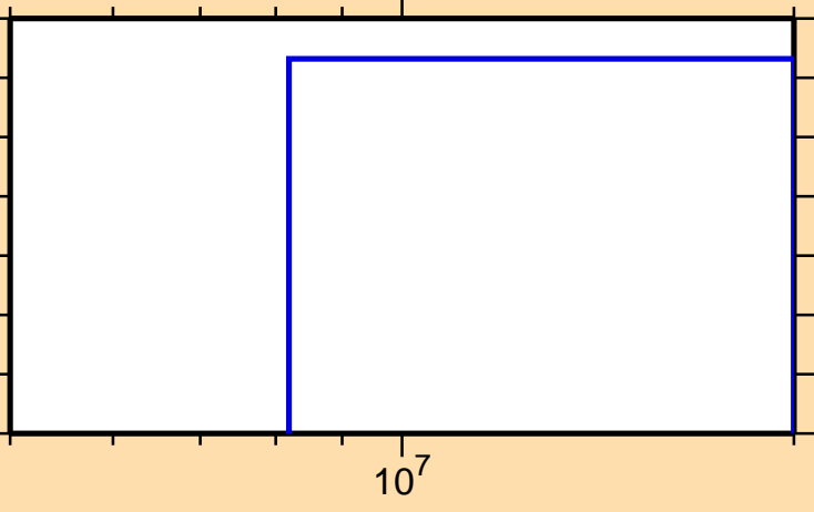
\sigma vs. E for ^{131}\text{Sb}(n,t)
