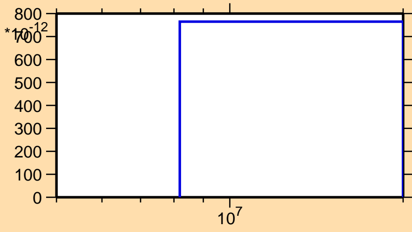
\sigma vs. E for ^{131}\text{Sb}(n,nd)
