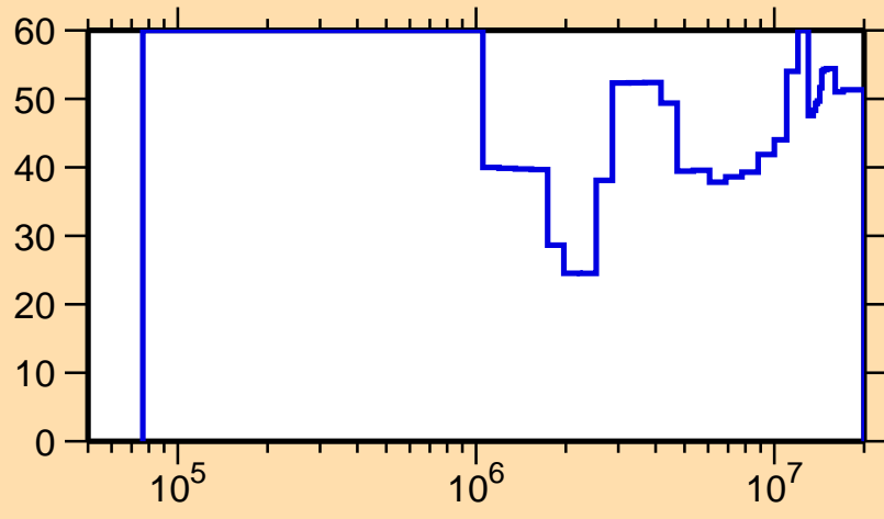
\Delta\sigma/\sigma vs. E for ^{132}\text{Sb}(n,n_1)
