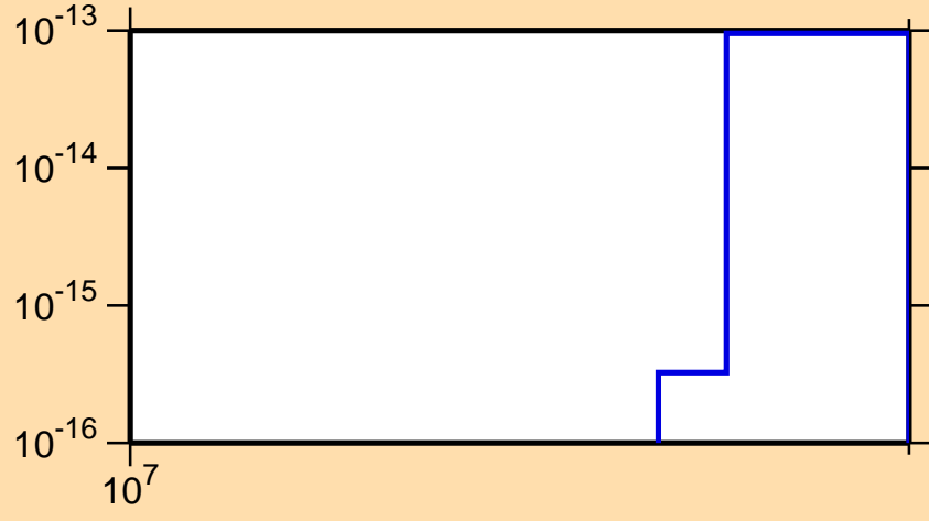
\sigma vs. E for ^{132}\text{Sb}(n,2n\alpha)
