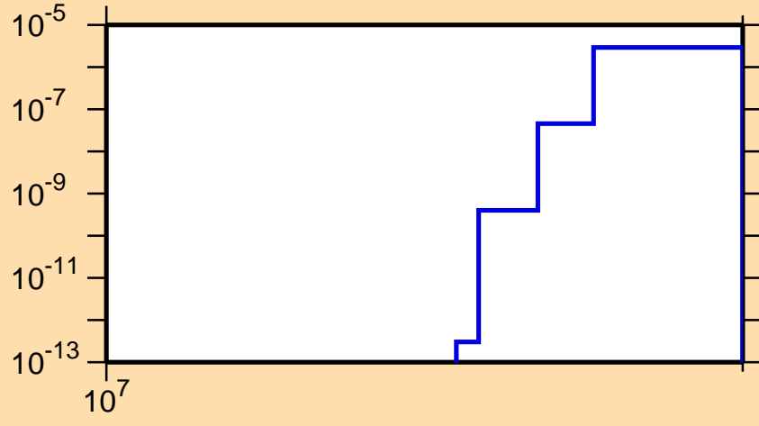
\sigma vs. E for ^{132}\text{Sb}(n,\text{nd})
