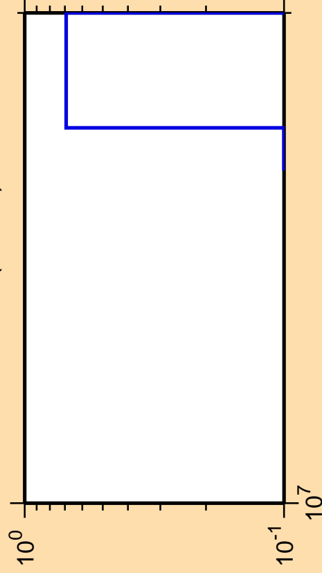
\Delta\sigma/\sigma vs. E for ^{132}\text{Sb}(n,2n\alpha)
