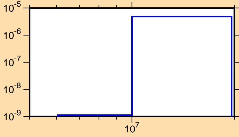
\sigma vs. E for ^{132}\text{Sb}(n,\alpha)
