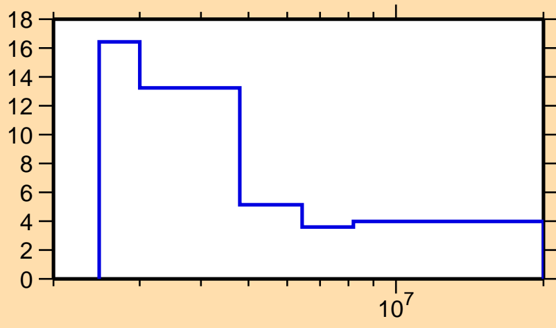
\Delta\sigma/\sigma vs. E for ^{132}\text{Sb}(n, tot.)
