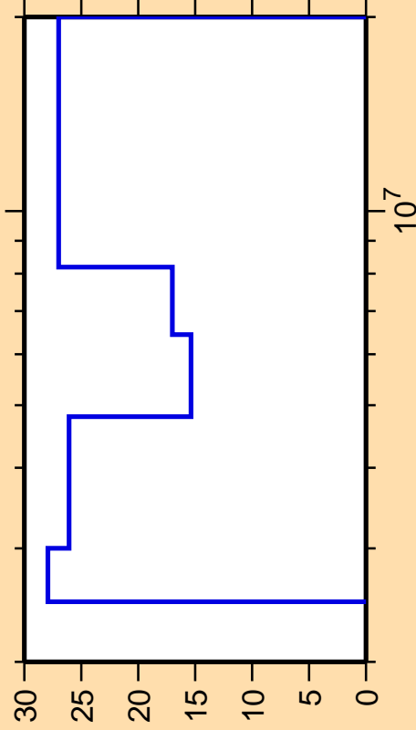
\Delta\sigma/\sigma vs. E for ^{132}\text{Sb}(n, ncont.)
