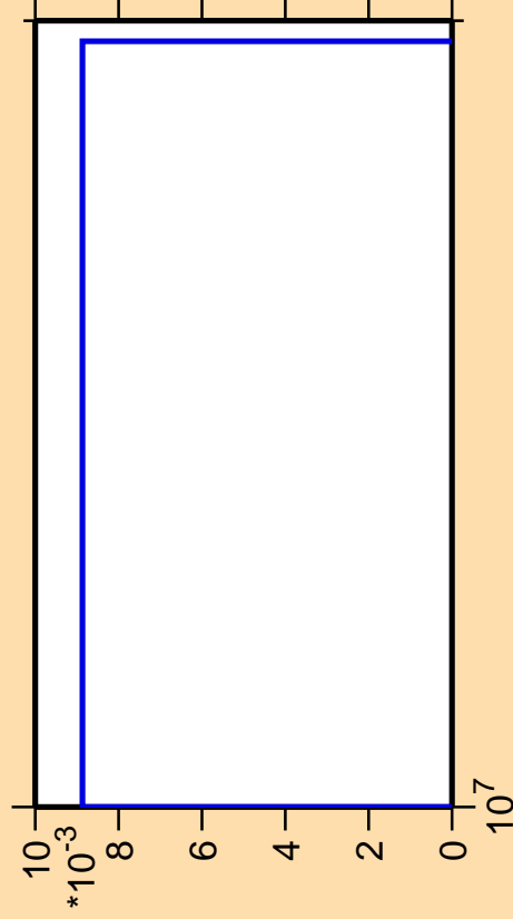
\Delta\sigma/\sigma vs. E for ^{132}\text{Sb}(n,2n\alpha)
