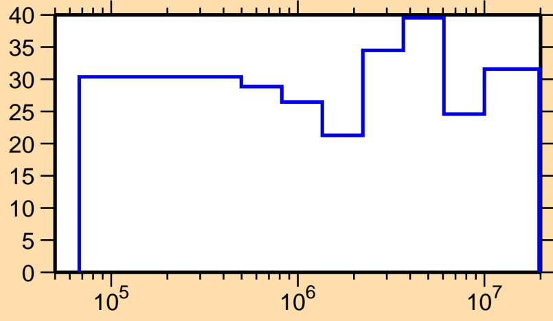
\Delta\sigma/\sigma vs. E for ^{132}\text{Sb}(n,n_1)
