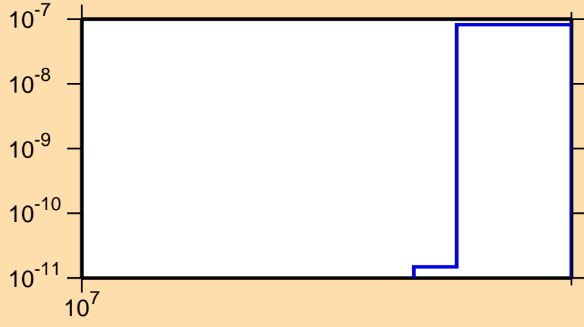
\sigma vs. E for ^{133}\text{Sb}(n,nt)
