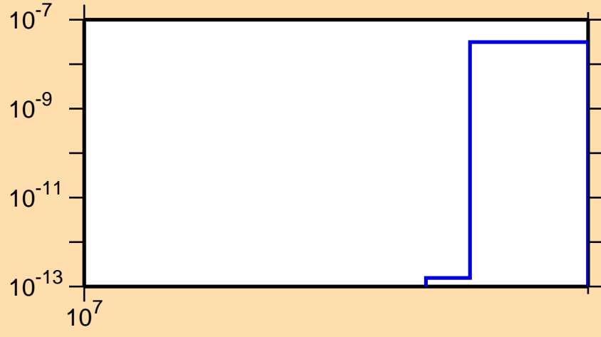
\sigma vs. E for ^{133}\text{Sb}(n,\text{nd})
