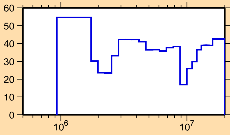
\Delta\sigma/\sigma vs. E for ^{133}\text{Sb}(n,n_1)
