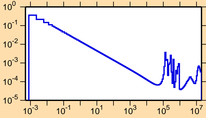
\sigma vs. E for ^{133}\text{Sb}(n,\gamma)
