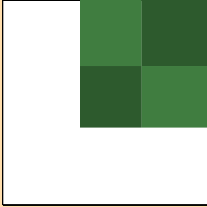
\sigma vs. E for ^{133}\text{Sb}(n,3n)
