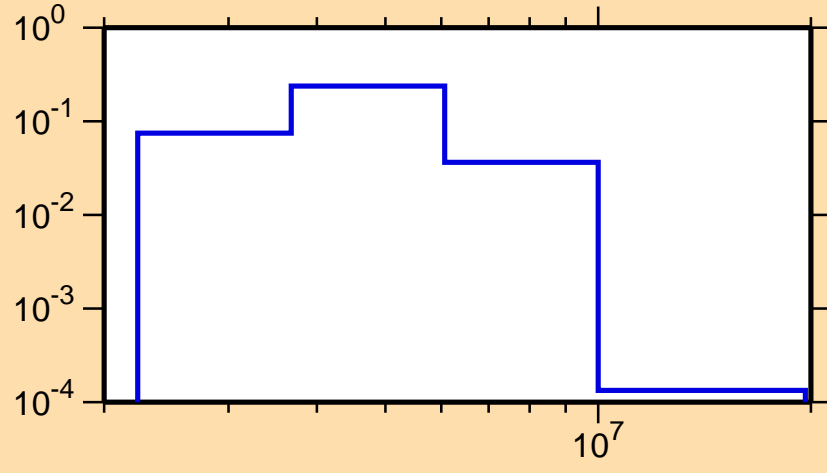
\sigma vs. E for ^{133}\text{Sb}(n,n_3)
