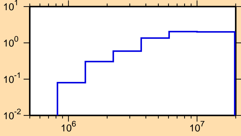
\sigma vs. E for ^{133}\text{Sb}(n,\text{nonel.})
