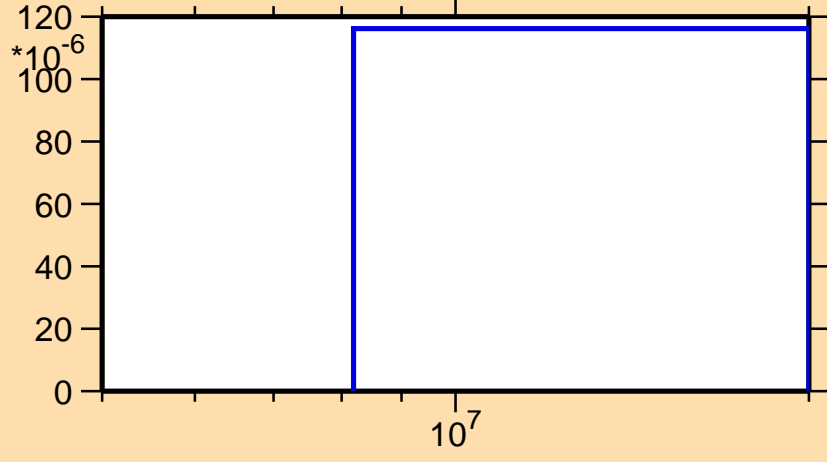
\sigma vs. E for ^{133}\text{Sb}(n,d)
