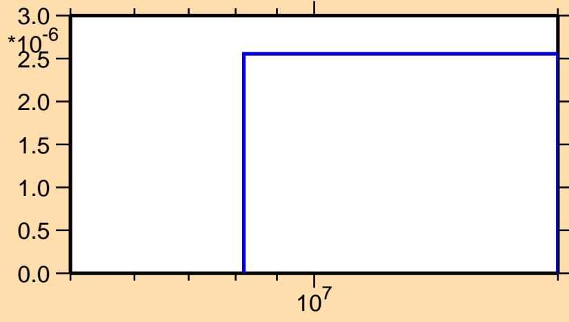
\sigma vs. E for ^{133}\text{Sb}(n,t)
