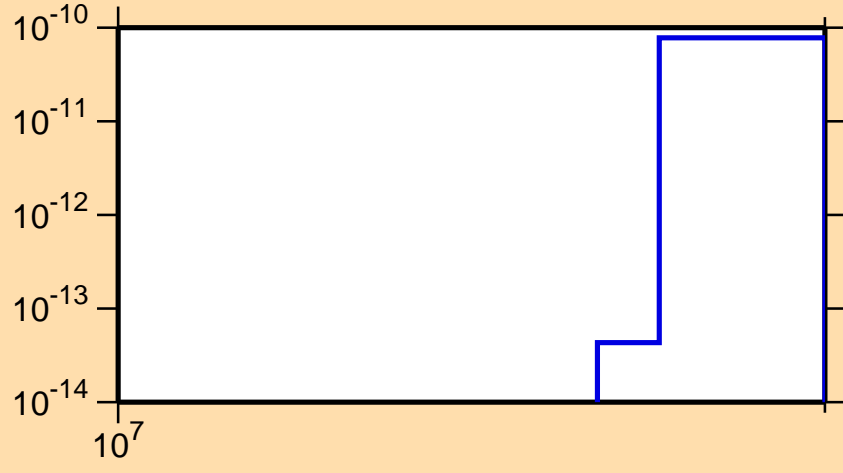
\sigma vs. E for ^{134}\text{Sb}(n,2n\alpha)
