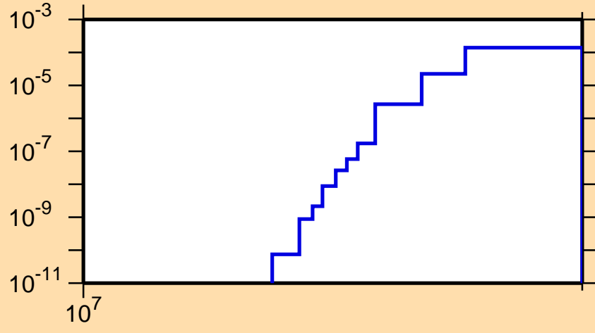
\sigma vs. E for ^{134}\text{Sb}(n,\text{nd})
