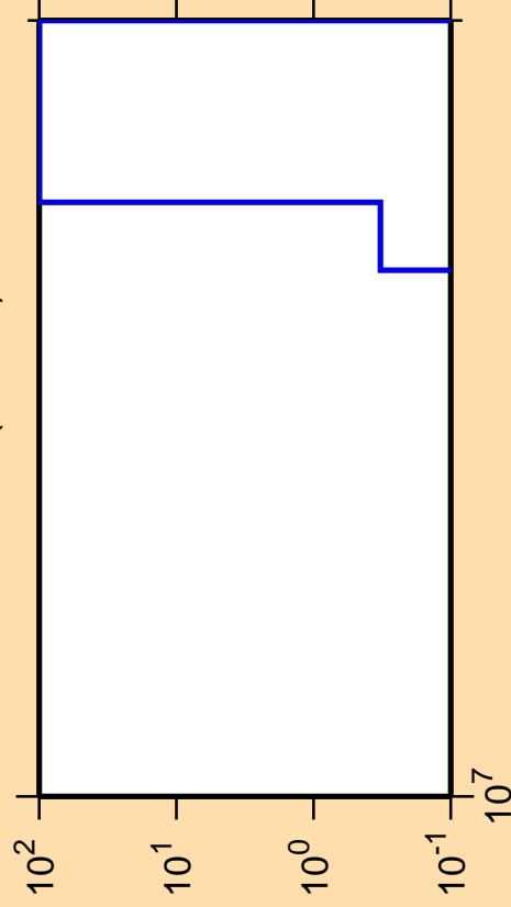
\Delta\sigma/\sigma vs. E for ^{134}\text{Sb}(n,2n\alpha)
