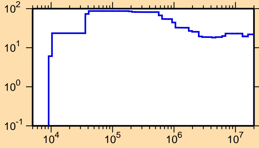
\Delta\sigma/\sigma vs. E for ^{134}\text{Sb}(n,\text{nonel.})
