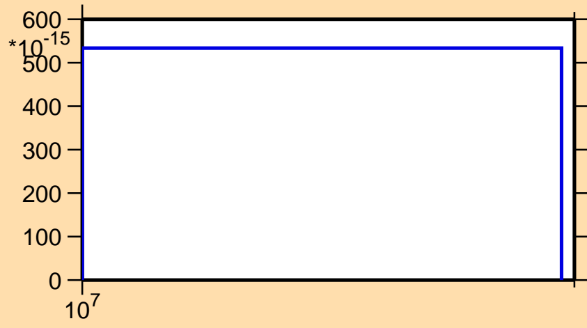
\sigma vs. E for ^{134}\text{Sb}(n,2n\alpha)
