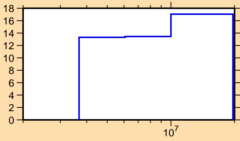
\Delta\sigma/\sigma vs. E for ^{134}\text{Sb}(n,\text{tot.})
