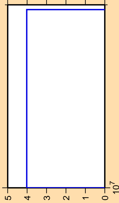
\Delta\sigma/\sigma vs. E for ^{134}\text{Sb}(n,2n\alpha)
