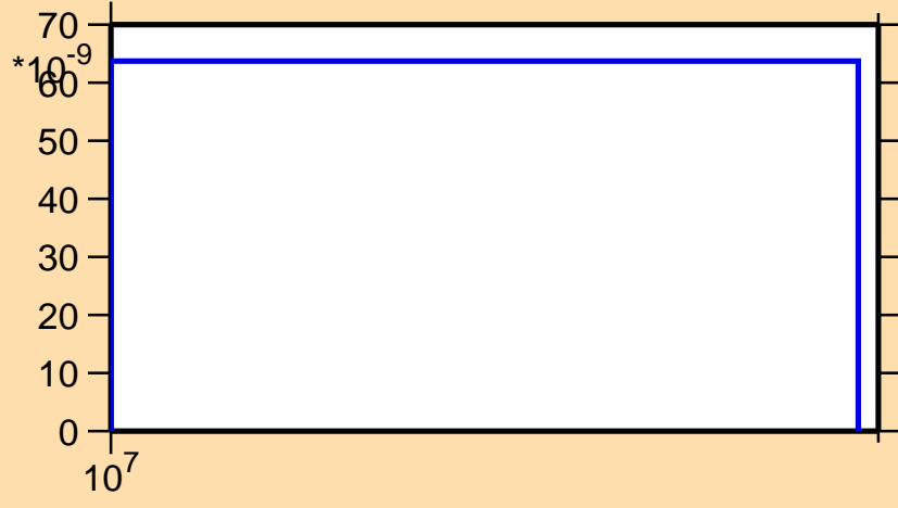
\sigma vs. E for ^{134}\text{Sb}(n,2np)
