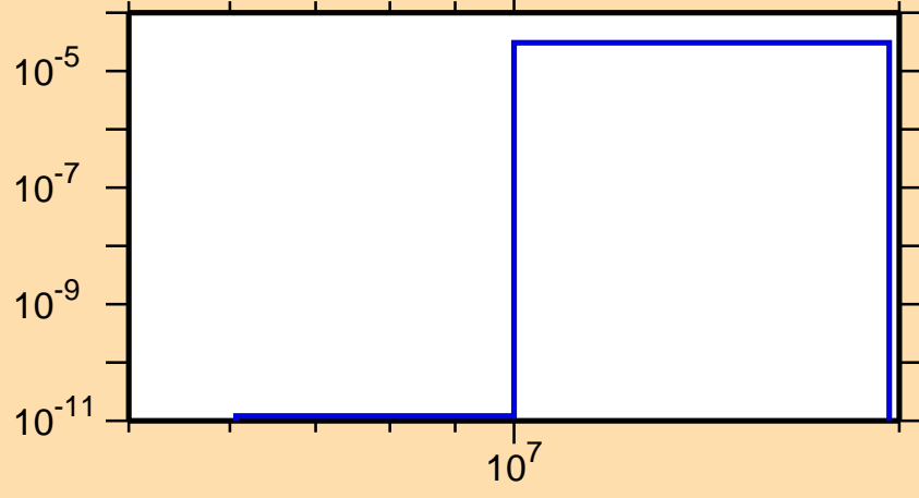
\sigma vs. E for ^{134}\text{Sb}(n,p)
