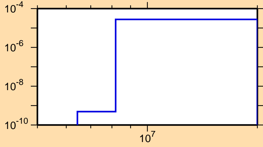
\sigma vs. E for ^{134}\text{Sb}(n,t)
