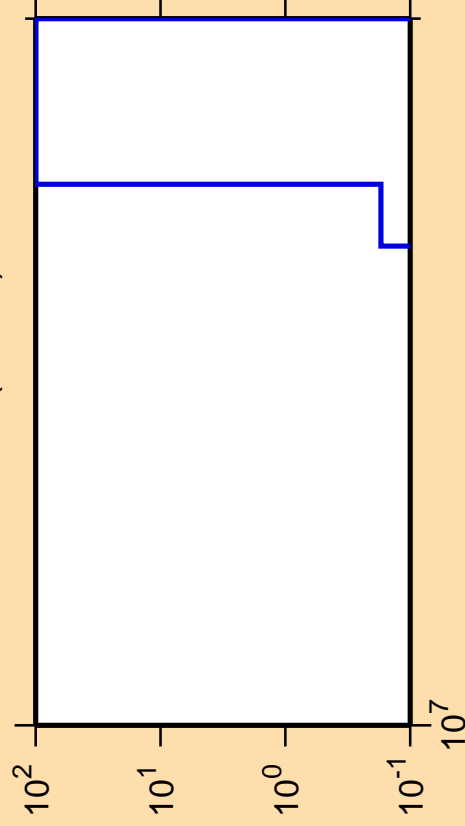
\Delta\sigma/\sigma vs. E for ^{135}\text{Sb} (mt 11)
