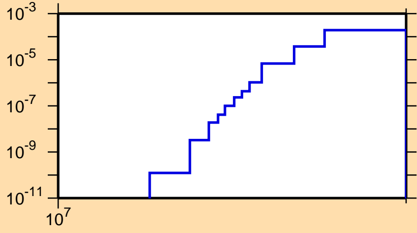
\sigma vs. E for ^{135}\text{Sb}(n,np)
