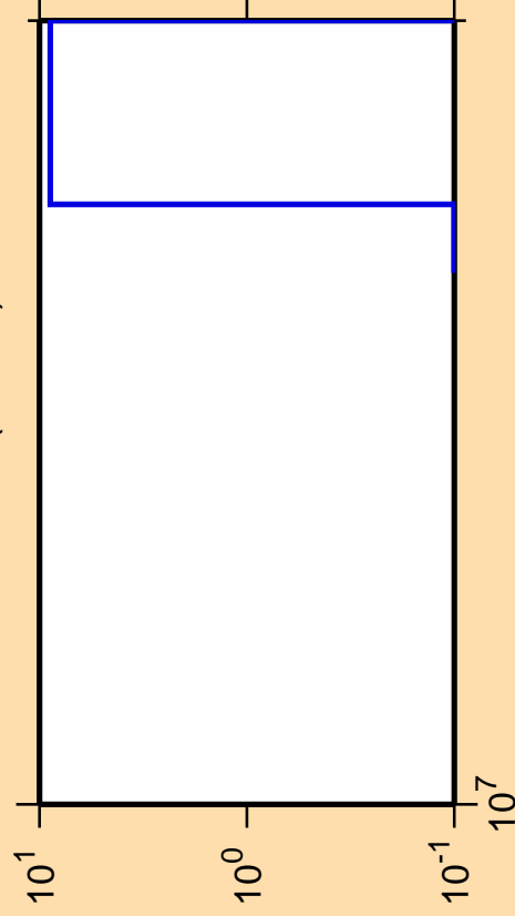
\Delta\sigma/\sigma vs. E for ^{135}\text{Sb} (mt 42)
