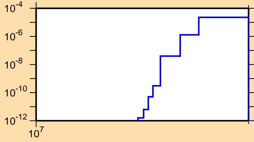
\sigma vs. E for ^{135}\text{Sb}(n,\text{nd})
