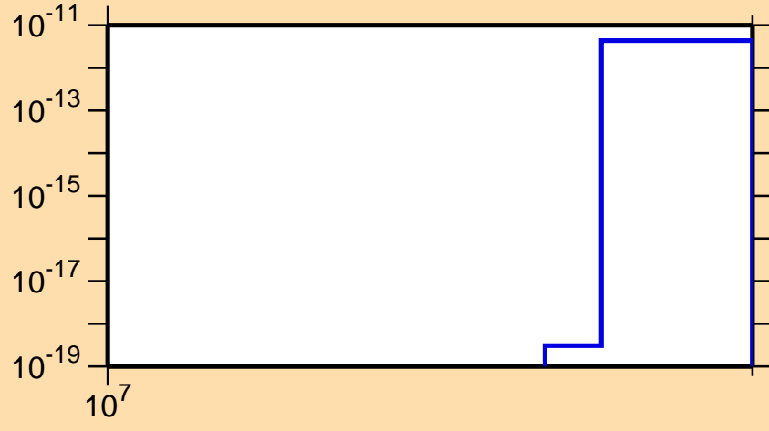
\sigma vs. E for ^{135}\text{Sb} (mt 42)
