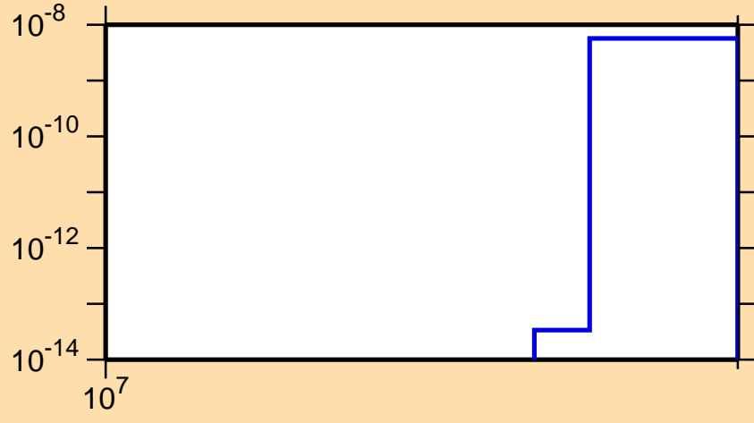
\sigma vs. E for ^{135}\text{Sb} (mt 11)
