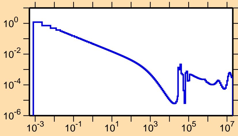
\sigma vs. E for ^{135}\text{Sb}(n,\gamma)
