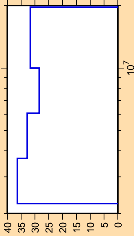
\Delta\sigma/\sigma vs. E for ^{135}\text{Sb}(n, n_{\text{cont}}) .
