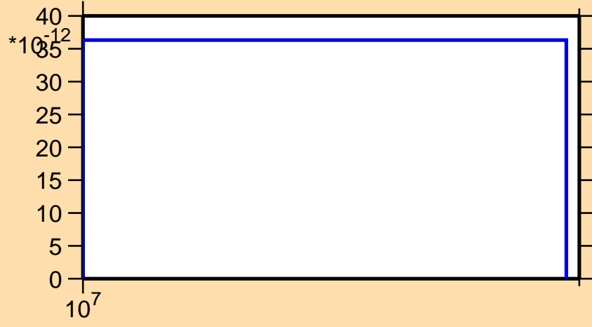
\sigma vs. E for ^{135}\text{Sb} (mt 11)
