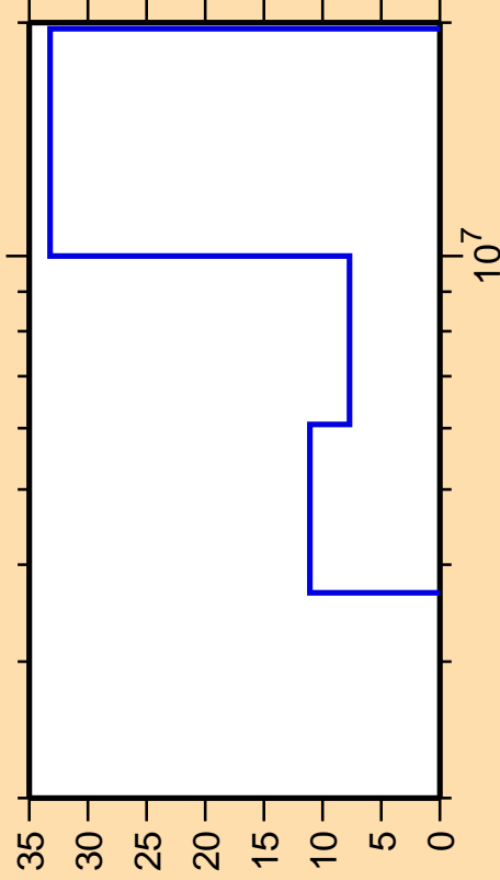
\Delta\sigma/\sigma vs. E for ^{135}\text{Sb}(n,2n)
