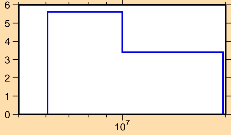
\Delta\sigma/\sigma vs. E for ^{135}\text{Sb}(n,\text{el.})
