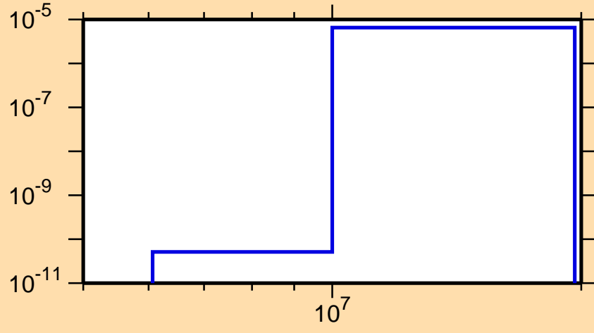
\sigma vs. E for ^{135}\text{Sb}(n,\alpha)
