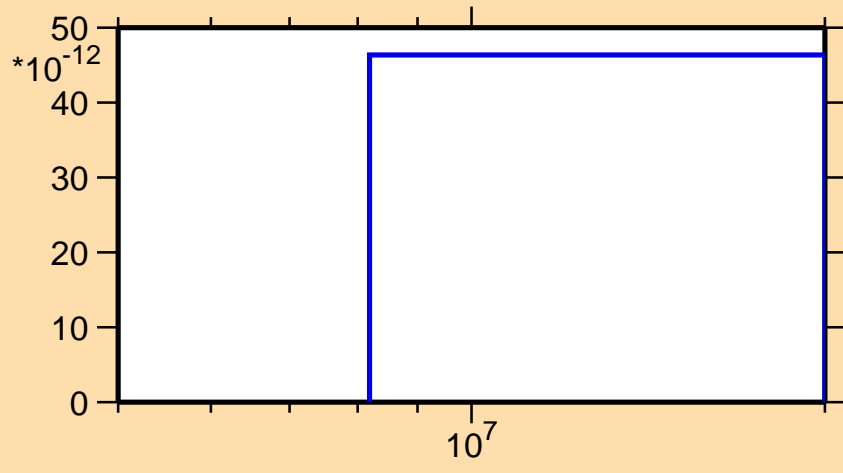
\sigma vs. E for ^{135}\text{Sb}(\text{mt } 11)
