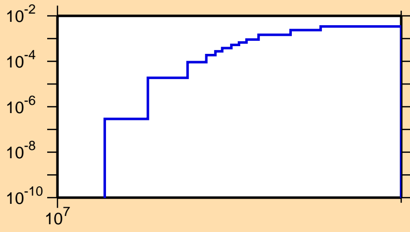
\sigma vs. E for ^{42}\text{Sc}(n,nd)
