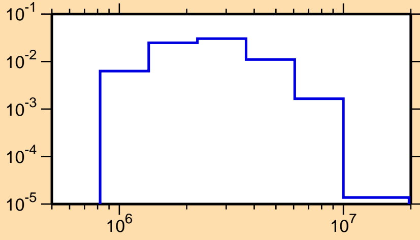
\sigma vs. E for ^{42}\text{Sc}(n,n_4)
