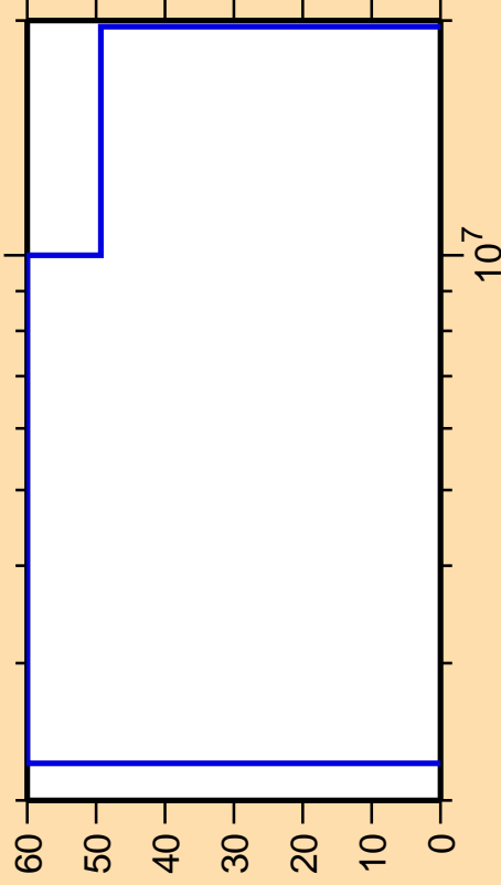
\Delta\sigma/\sigma vs. E for ^{42}\text{Sc}(n,n\text{cont.})
