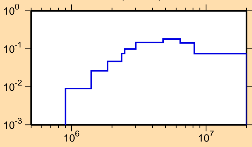
\sigma vs. E for ^{42}\text{Sc}(n,\text{inel.})
