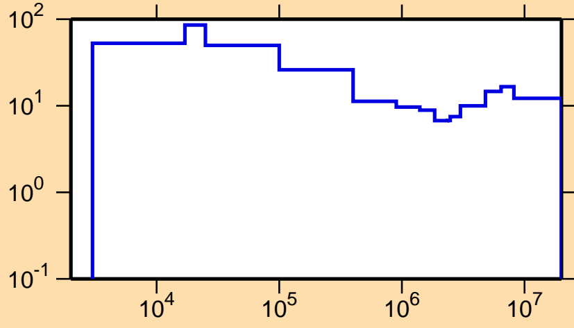
\Delta\sigma/\sigma vs. E for ^{42}\text{Sc}(n,el.)
