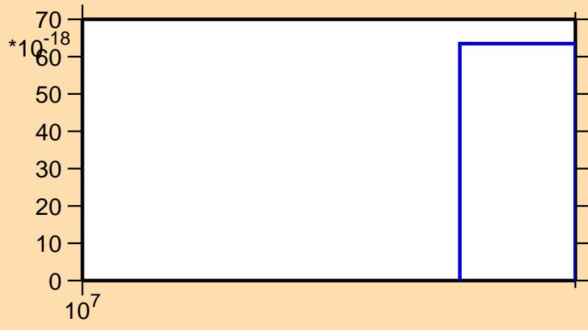
\sigma vs. E for ^{43}\text{Sc}(n,2n\alpha)
