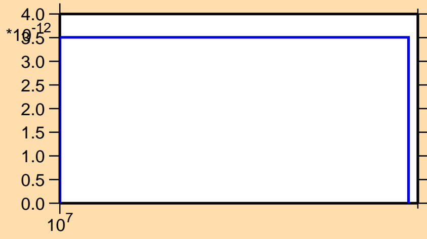
\sigma vs. E for ^{43}\text{Sc}(n,\text{pt})
