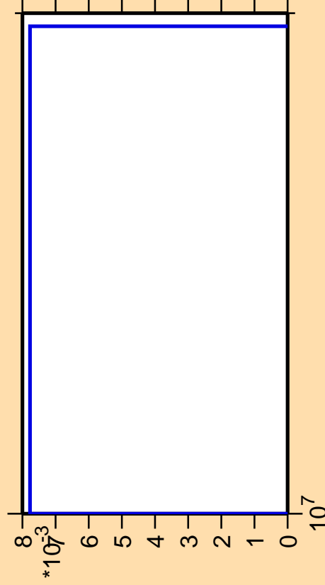
\Delta\sigma/\sigma vs. E for ^{43}\text{Sc} (mt 34)
