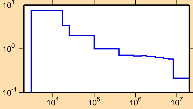
\sigma vs. E for ^{43}\text{Sc}(n,p)
