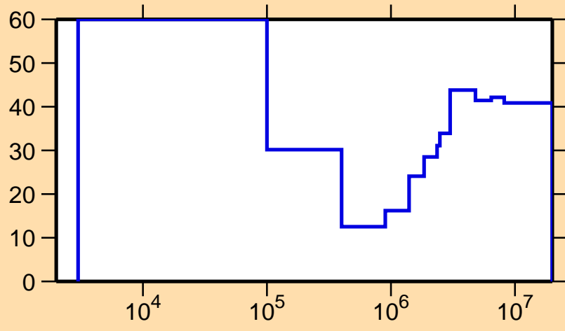
\Delta\sigma/\sigma vs. E for ^{43}\text{Sc}(n,p)
