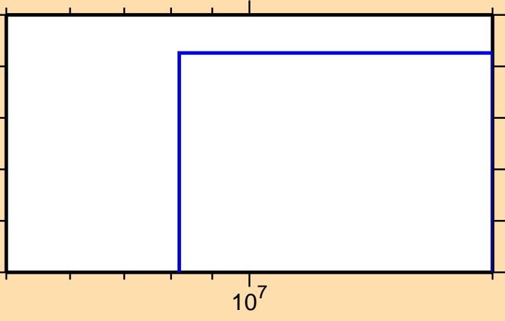
\sigma vs. E for ^{43}\text{Sc}(n,\text{nd})
