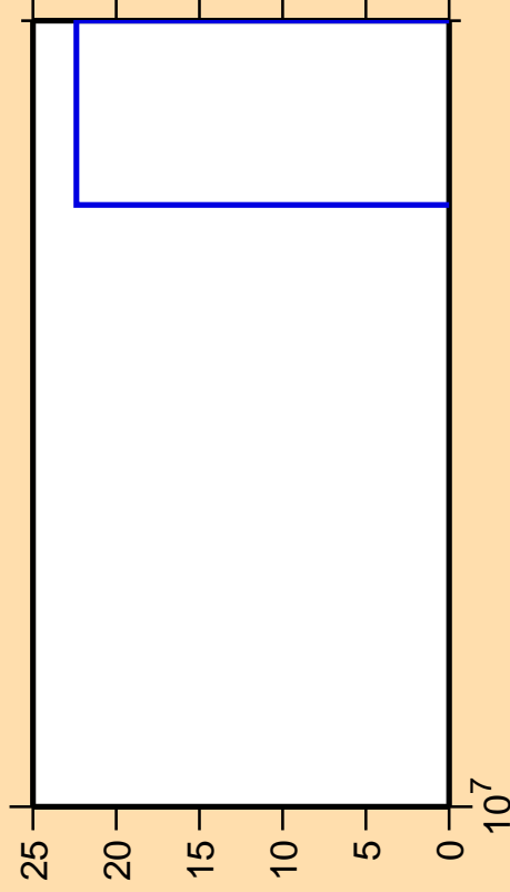
\Delta\sigma/\sigma vs. E for ^{44}\text{Sc} (mt 34)
