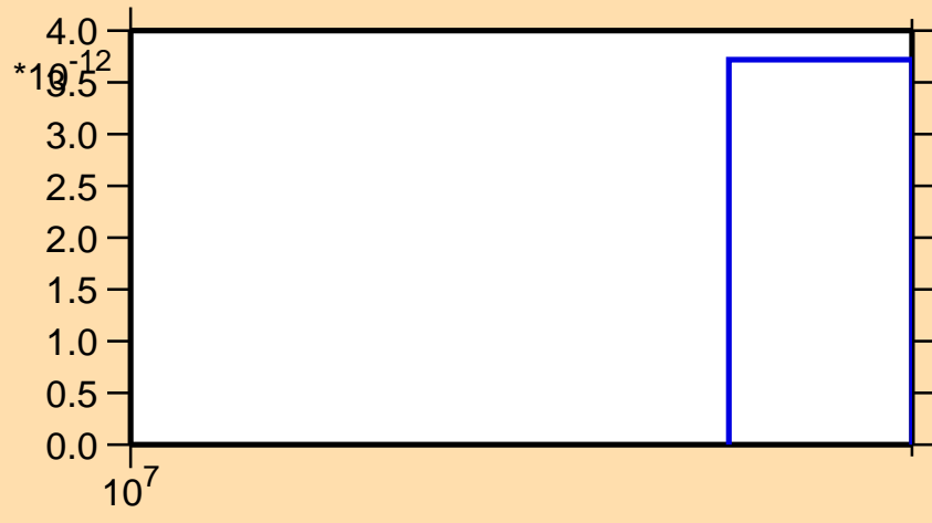
\sigma vs. E for ^{44}\text{Sc} (mt 34)
