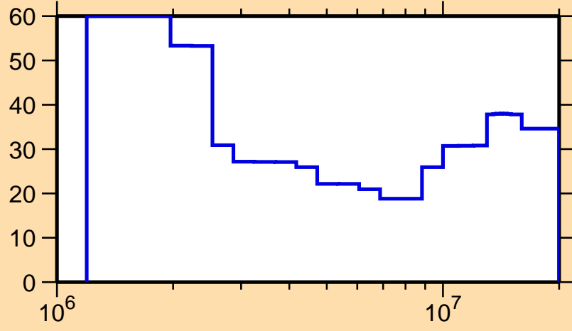
\Delta\sigma/\sigma vs. E for ^{44}\text{Sc}(n,n\text{cont.})
