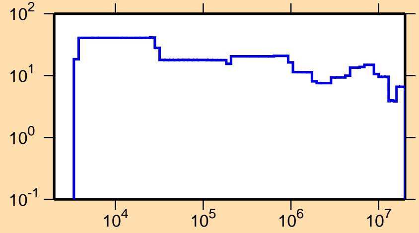
\Delta\sigma/\sigma vs. E for ^{44}\text{Sc}(n,\text{el.})
