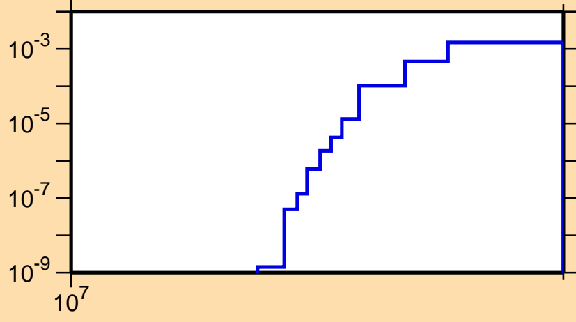
\sigma vs. E for ^{44}\text{Sc}(n,\text{nd})
