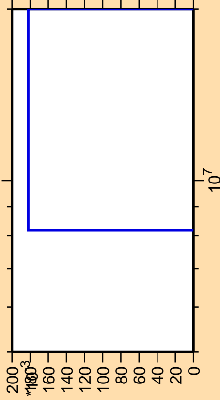
\Delta\sigma/\sigma vs. E for ^{44}\text{Sc} (mt 34)
