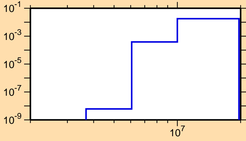
\sigma vs. E for ^{45}\text{Sc}(n,d)
