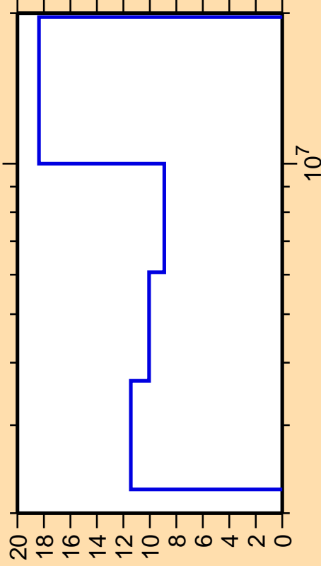
\Delta\sigma/\sigma vs. E for ^{45}\text{Sc}(n,n_{\text{cont}})
