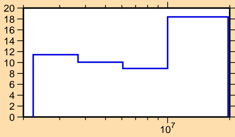
\Delta\sigma/\sigma vs. E for ^{45}\text{Sc}(n,n\text{cont.})
