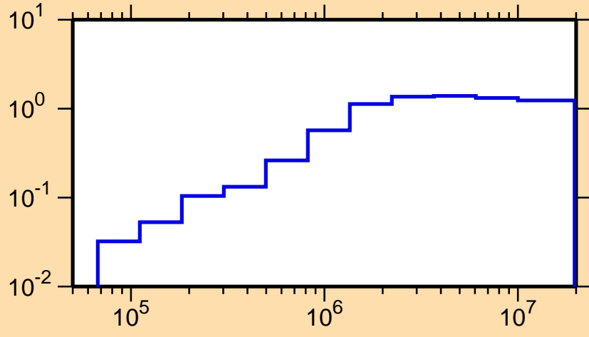
\sigma vs. E for ^{45}\text{Sc}(n,\text{nonel.})
