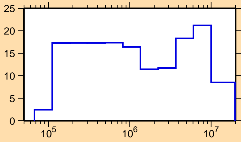
\Delta\sigma/\sigma vs. E for ^{45}\text{Sc}(n,el.)
