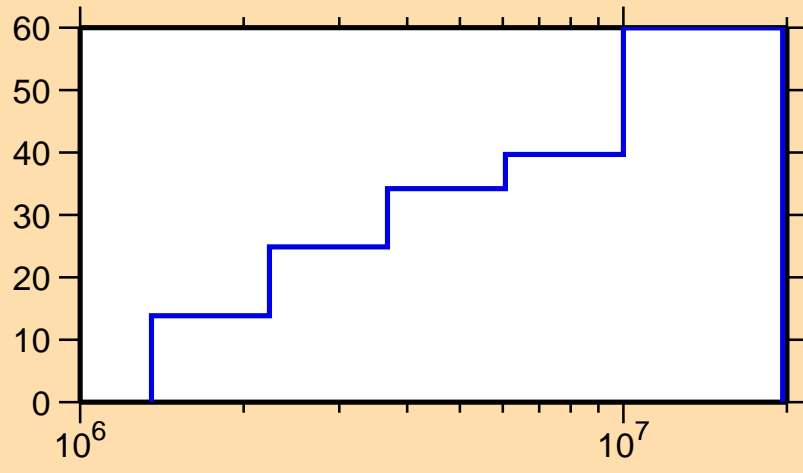
\Delta\sigma/\sigma vs. E for ^{45}\text{Sc}(n,n_1)
